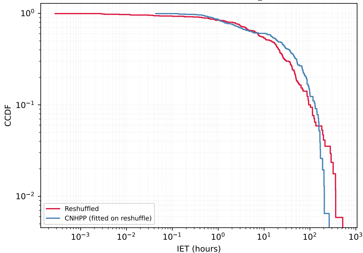
User 32432053 - Reshuffled vs CNHPP A_{\text{fit}}=0.3166
